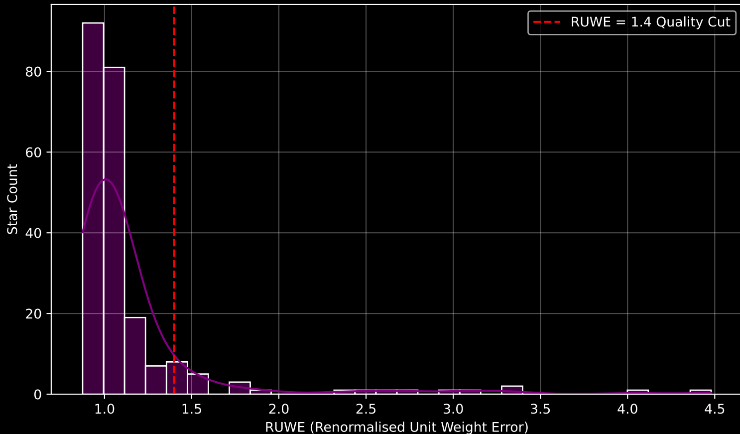
GALAH DR4 Field [8340] RUWE Distribution (n= 226)
