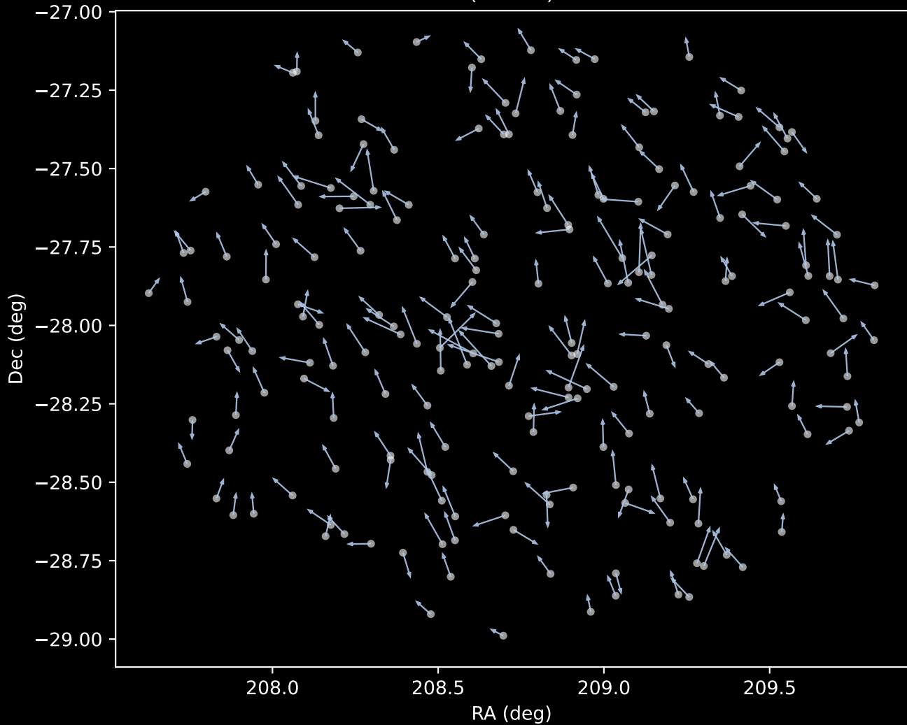
GALAH DR4 Cluster 1 Proper Motion Vectors (n=203)
