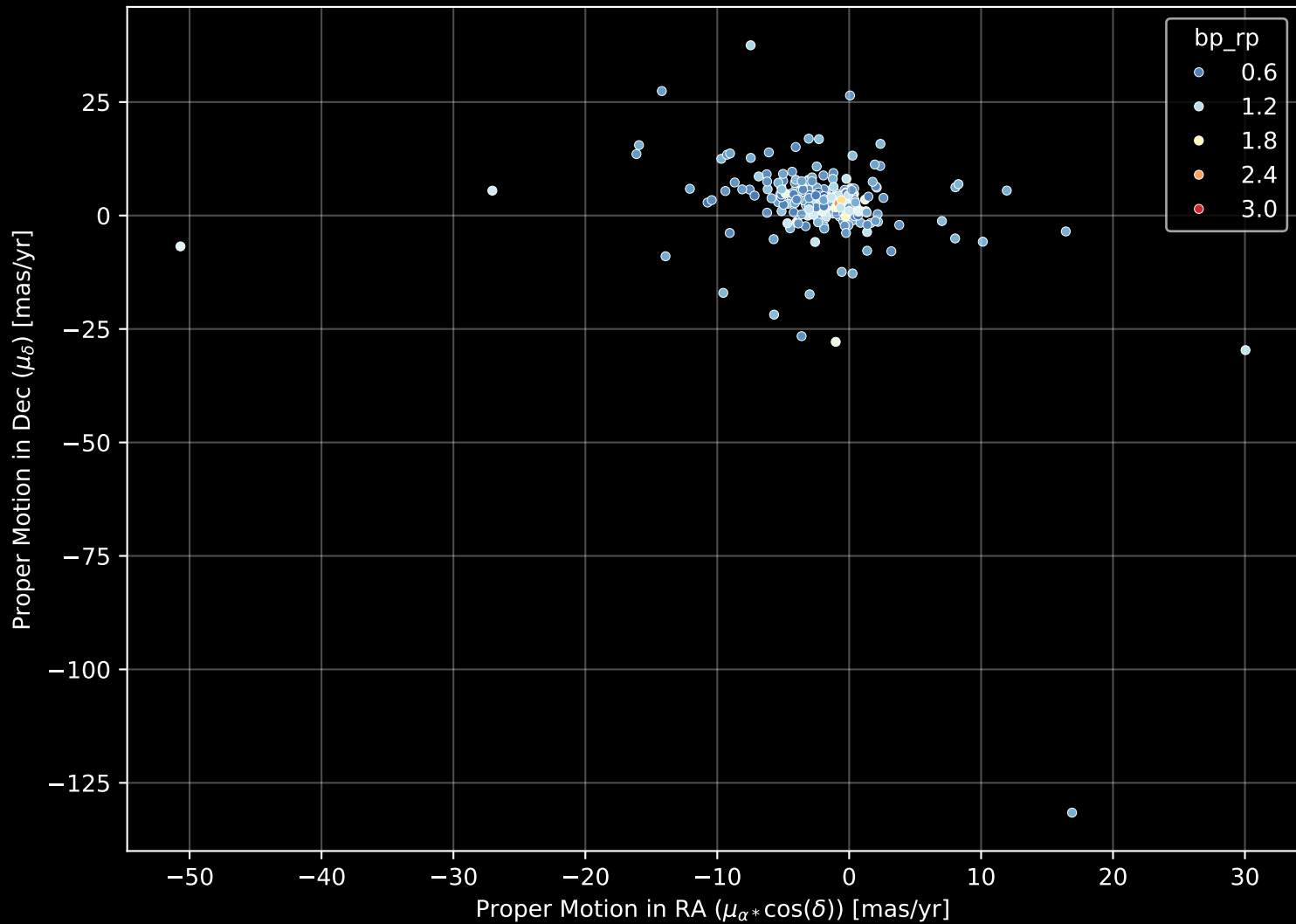
GALAH DR4 Field: [8340] Proper Motion Diagram (n= 239)
