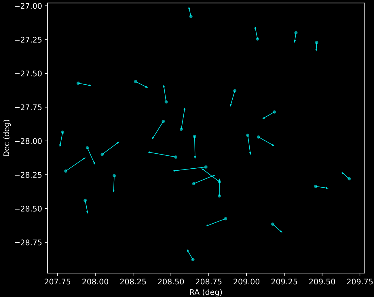
GALAH DR4 Noise Stream Proper Motion Vectors (n=30)
