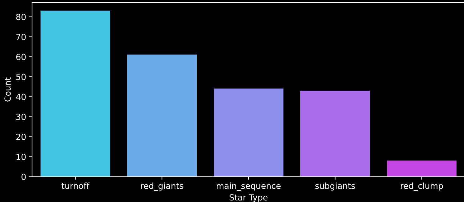
GALAH DR4 Field: [8340] Count plot of Star Type
